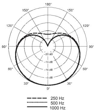
Polar Pattern
