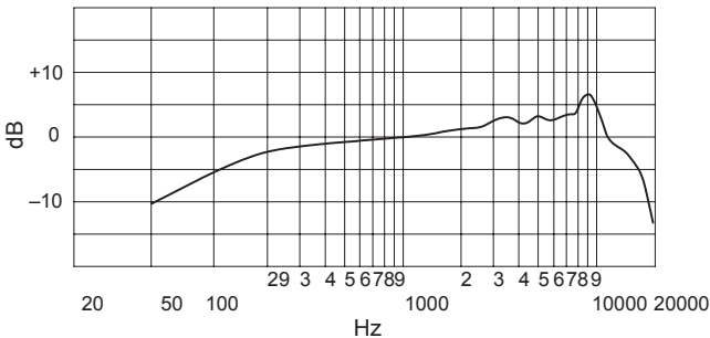
Frequency Response
