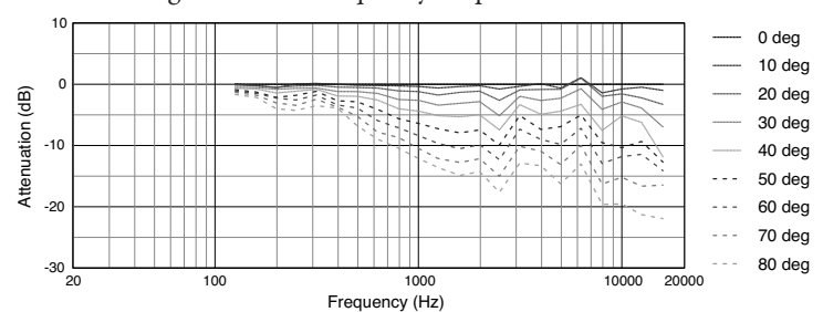
Vertical Up Off-Axis Frequency Response
